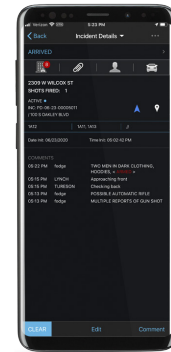
iOS Dashboard
